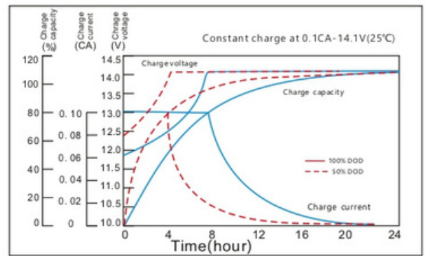
Charging characteristic
